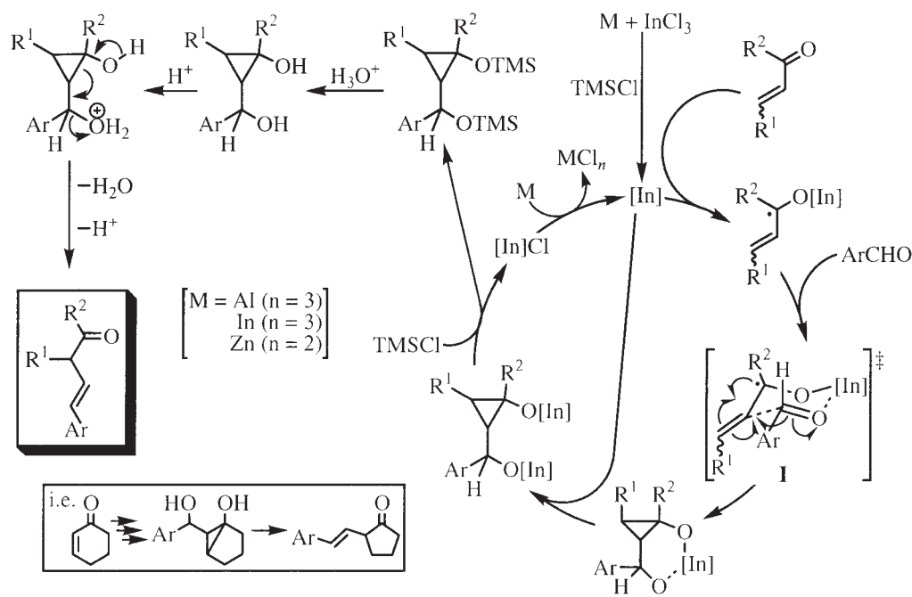
Scheme 4. Plausible reaction pathway.
